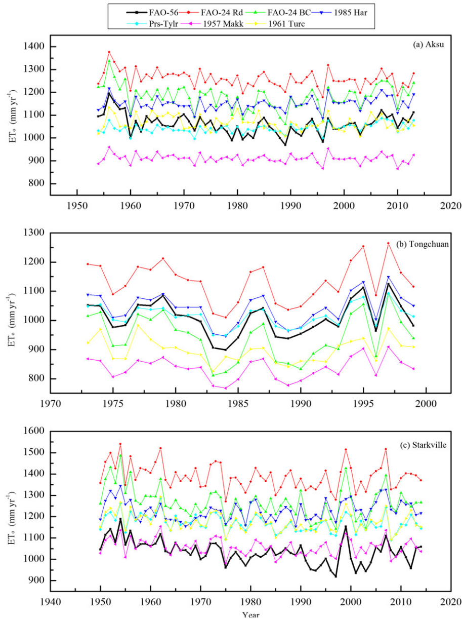
FIGURE 8. Comparison of Total Annual ET_0 by Six Alternative Simple Methods vs. FAO-56 Method at an Arid Region (Aksu), a Semiarid Region (Tongchuan), and a Humid Region (Starkville).
