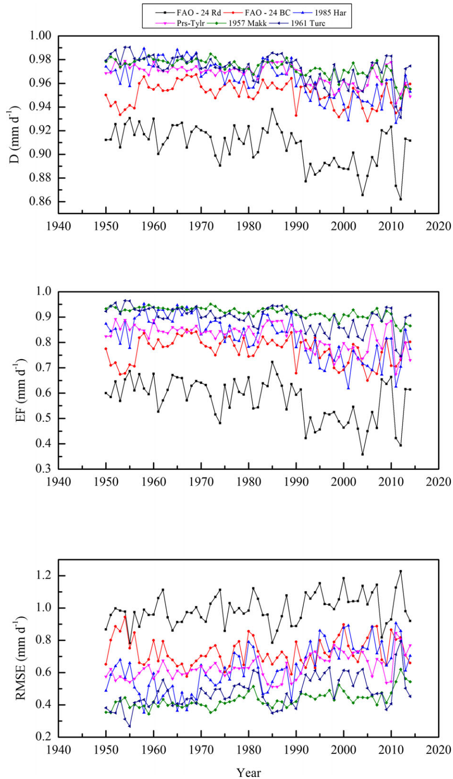
FIGURE 7. Monthly Averages of Daily ET_0 , Temporal Variation of D , EF , Root Mean Square Error ( RMSE ) for Different ET_0 Methods at a Humid Region (Starkville).
