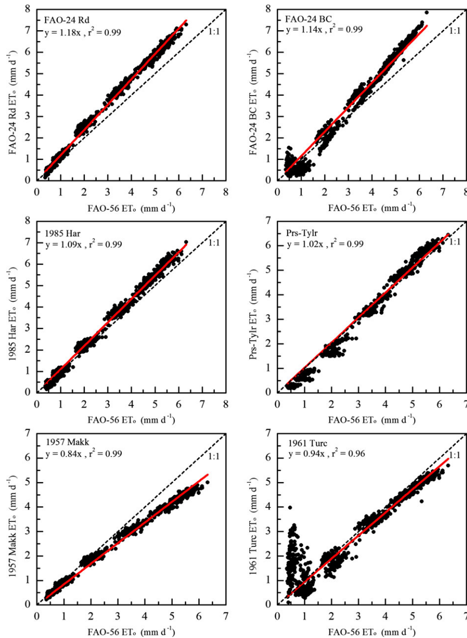
FIGURE 2. Monthly Averages of Daily ET_0 Calculated by Six Alternative Methods vs. FAO-56 Method in an Arid Region (Aksu).
