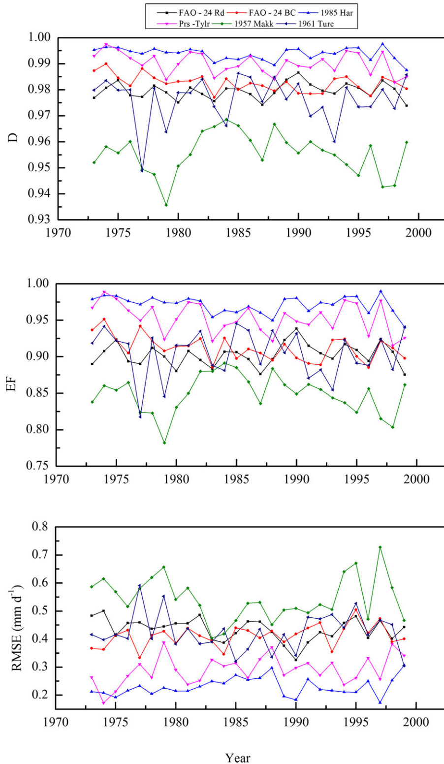
FIGURE 5. Temporal Variation of Comparison Statistics ( D , EF , root mean square error [RMSE]) on Monthly Averages of Daily ET_0 for Different Methods at a Semiarid Region (Tongchuan).
