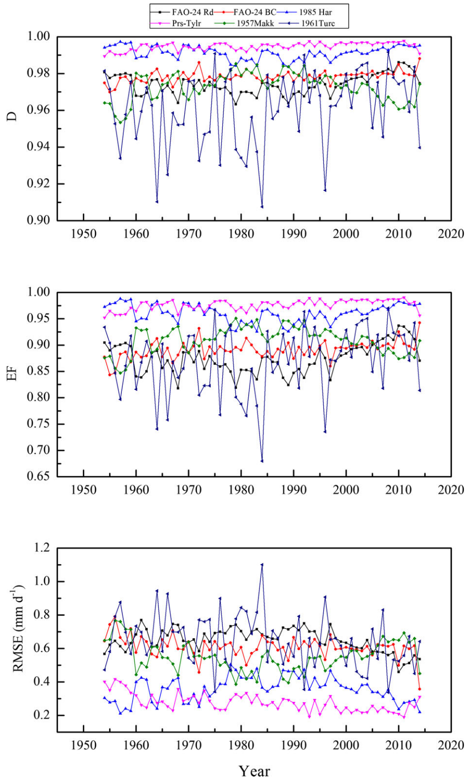
FIGURE 3. Temporal Variation of Comparison Statistics ( D , EF , root mean square error [RMSE]) on Monthly Averages of Daily ET_o for Different Methods in an Arid Region (Aksu).
