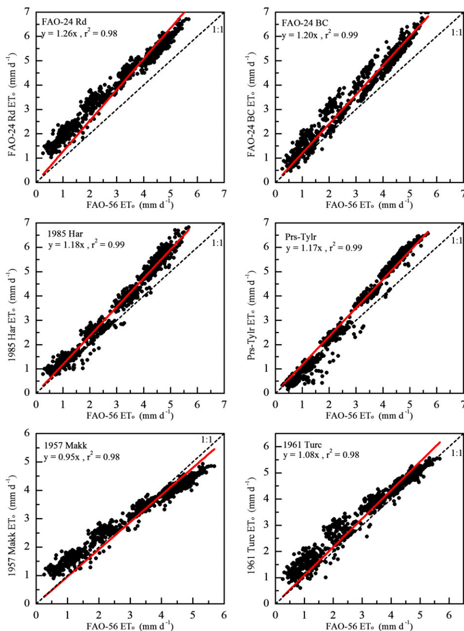
FIGURE 6. Monthly Averages of Daily ET_0 Calculated by Six Alternative Methods vs. FAO-56 Method in a Humid Region (Starkville).
