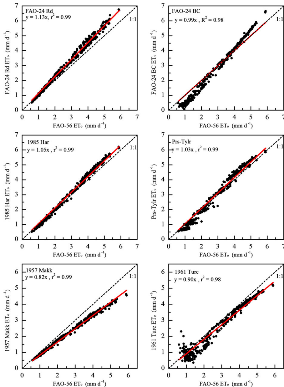
FIGURE 4. Monthly Averages of Daily ET_0 Calculated by Six Alternative Methods vs. FAO-56 Method in a Semiarid Region (Tongchuan).
