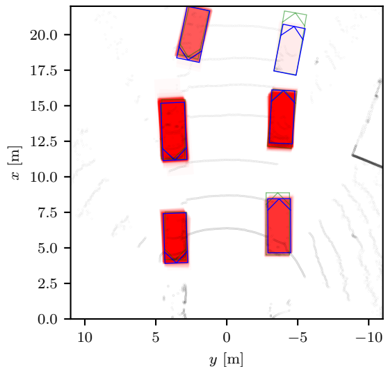
Fig. 4. Detection example using a simulated VLP-32 range image based on KITTI data. Raw detections after applying the threshold are displayed as opaque red boxes (darker red implies more overlapping detections). Objects after non-maximum suppression are shown in blue. The labels are visible in green.
