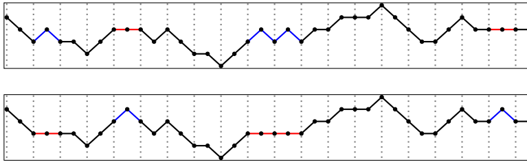
FIG 2. The partition into two-step segments is represented by dashed gray lines. type 2 segments are red, and type 3 segments are blue. The two paths represent S^0 and \hat{S}^0 , as related to each other by the permutation of type 2 and 3 segments.
