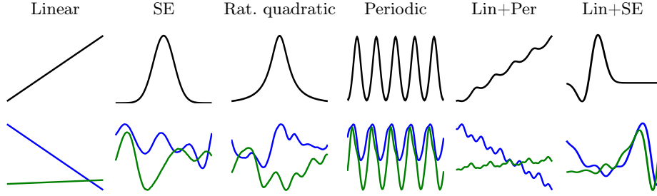
Fig. 2. Base kernels (top) and two random draws from a GP with each respective kernel and combination of kernels (bottom).
