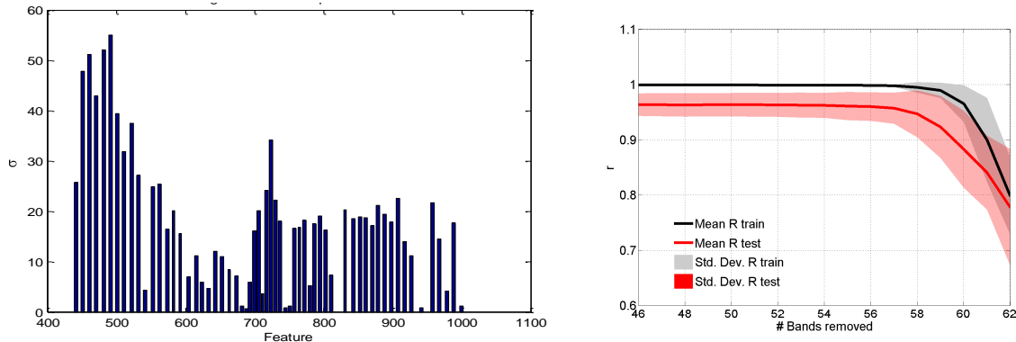
Fig. 4. Estimated \sigma_b values for one GP model using 62 CHRIS bands (left). The lower the \sigma_b the more important the band is for regression. Chl r and standard deviation (SD) of training and validation for GP fittings using backward elimination (right).
