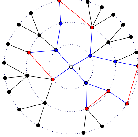
Figure 5.2. Graphical representation of the proof of (5.25). We draw the ball B_r for r = 3 . The spanning tree T is drawn using black and blue edges, and the spheres of radii 1, 2, 3 are drawn using dots. The red edges are E_1 , the blue edges E_2 , the red vertices U_1 , and the blue vertices U_2 \setminus U_1 .
