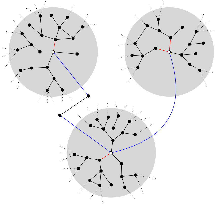
Figure 7.1. A schematic illustration of the algorithm in the proof of Lemma 7.2. The vertices of \mathcal{V} are white and the other vertices black. The balls B_{r_{x,\tau}}(x) , for each x \in \mathcal{V} , are indicated using grey balls, and they are disjoint by construction. The edges of the subgraph H^{(1)} are drawn in red. The edges of the subgraph H^{(2)} are drawn in blue.
