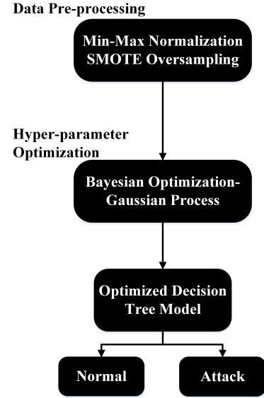
Fig. 1. Proposed Optimized IoT Botnet Detection Framework
