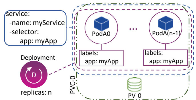
Fig. 2. Deploying stateful applications with Deployment controllers.
