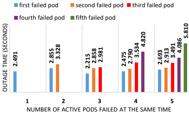
Fig. 7. Service Outage of simultaneously failed pods – The SC integrated with a StatefulSet controller (RQ4).
