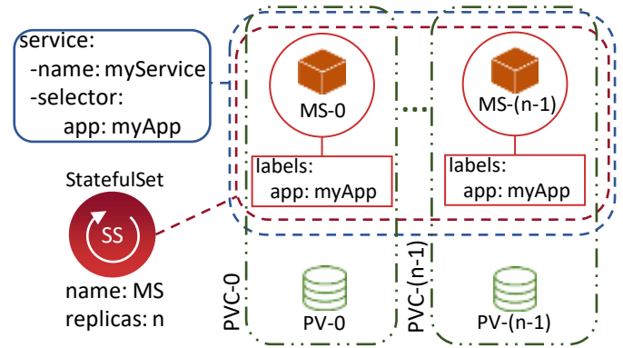
Fig. 1. Deploying stateful applications with StatefulSet controllers.
