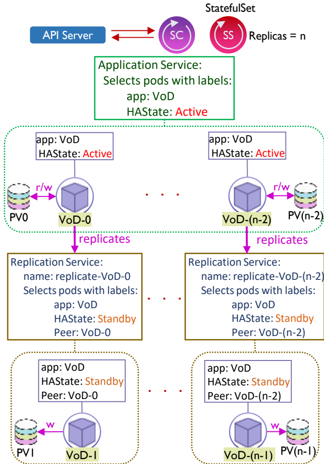
Fig. 4. Integrating the State Controller with StatefulSet controllers.
