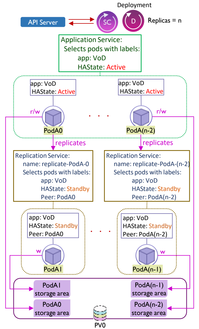
Fig. 5. Integrating the HA State Controller with Deployment controllers.
