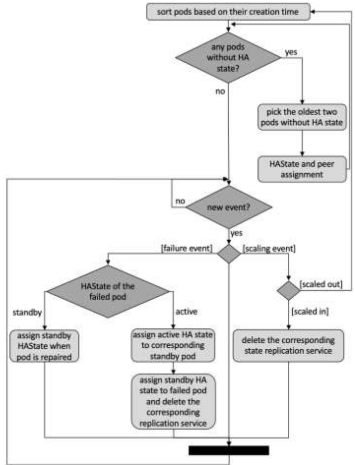
Fig. 3. Activity diagram of the HA State Controller.
