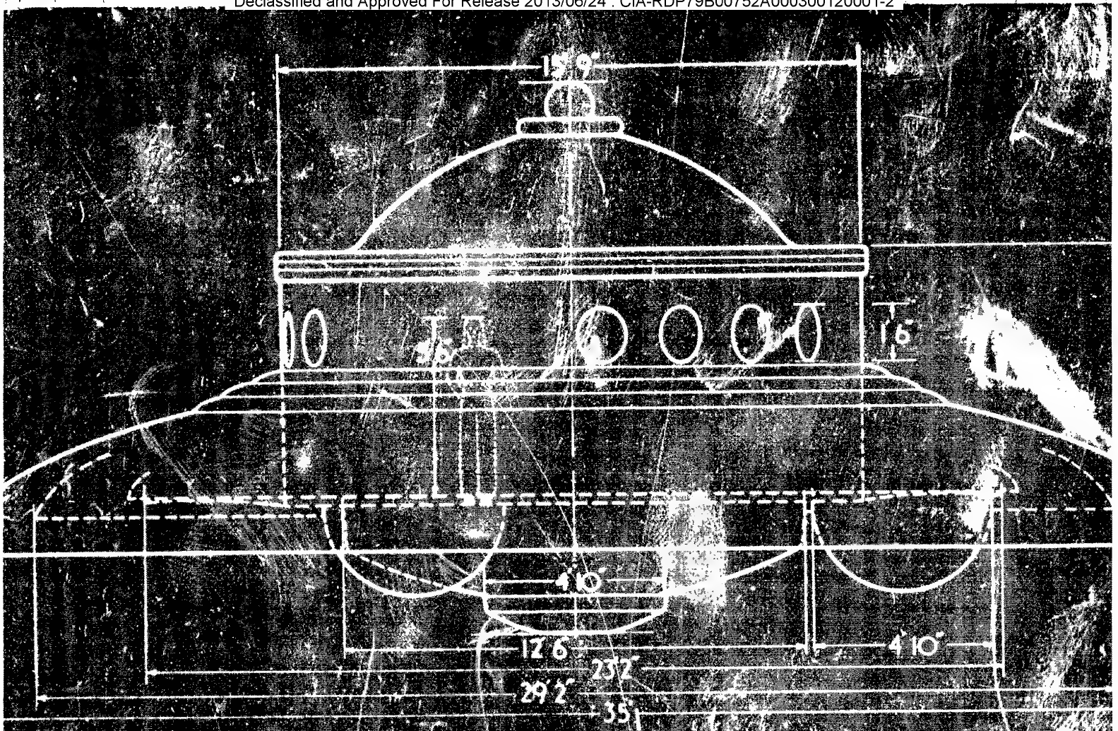
15b Major dimensions of flying saucer, obtained by analysis of the Adamski
