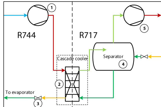
Figure 1.4: Cascade cooler
