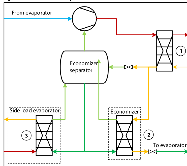
Figure 1.2: Side load evaporator
