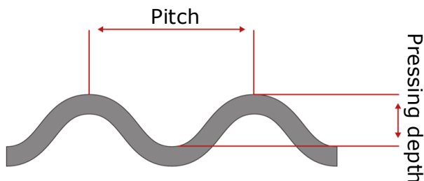
Figure 1.17: Plate corrugation
