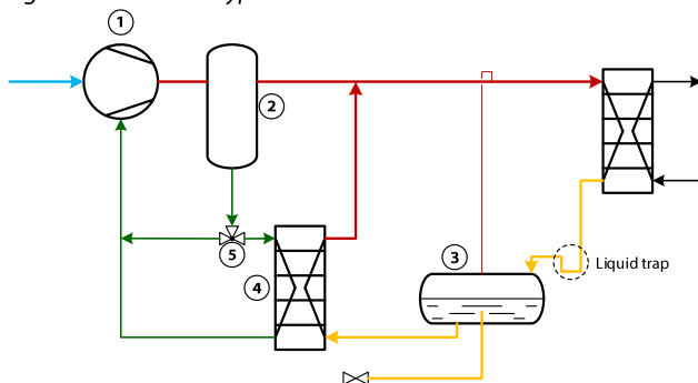
Figure 1.26: Thermosyphon oil cooler
