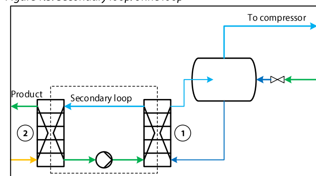
Figure 1.5: Secondary loop/brine loop
