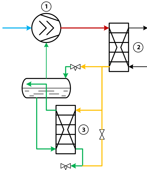
Figure 1.28: Closed economizer
