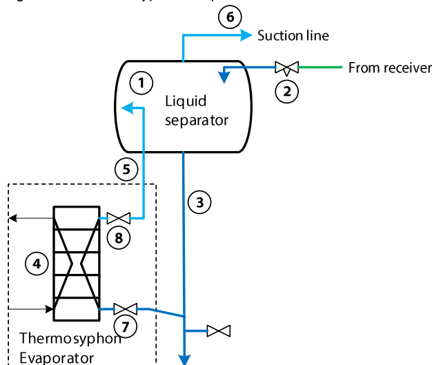
Figure 1.20: Thermosyphon evaporator
