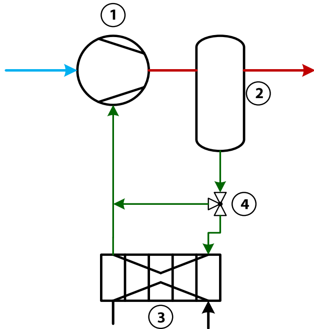
Figure 1.25: Brine/water cooled oil cooler
