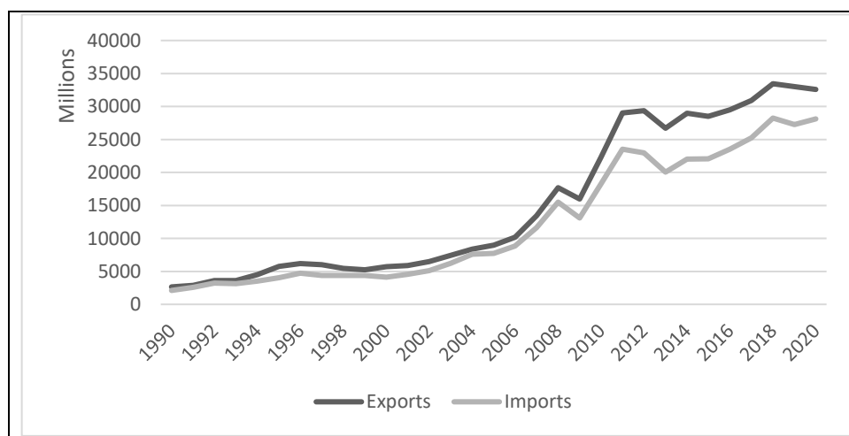
Figure 1: Intra-ASEAN Agri-Food Trade, 1990-2020 (USD million)
