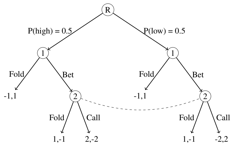
Figure 9: A simplified Poker game
