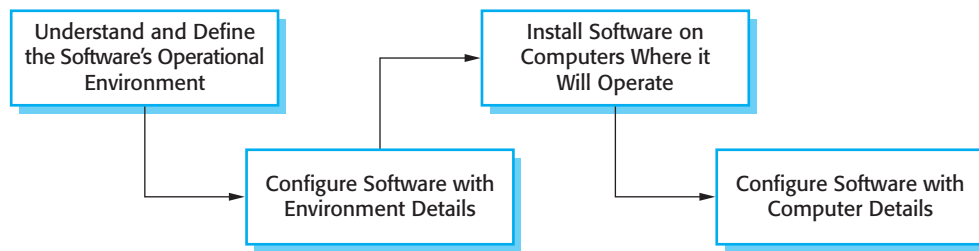
Figure 14.7 Software deployment
