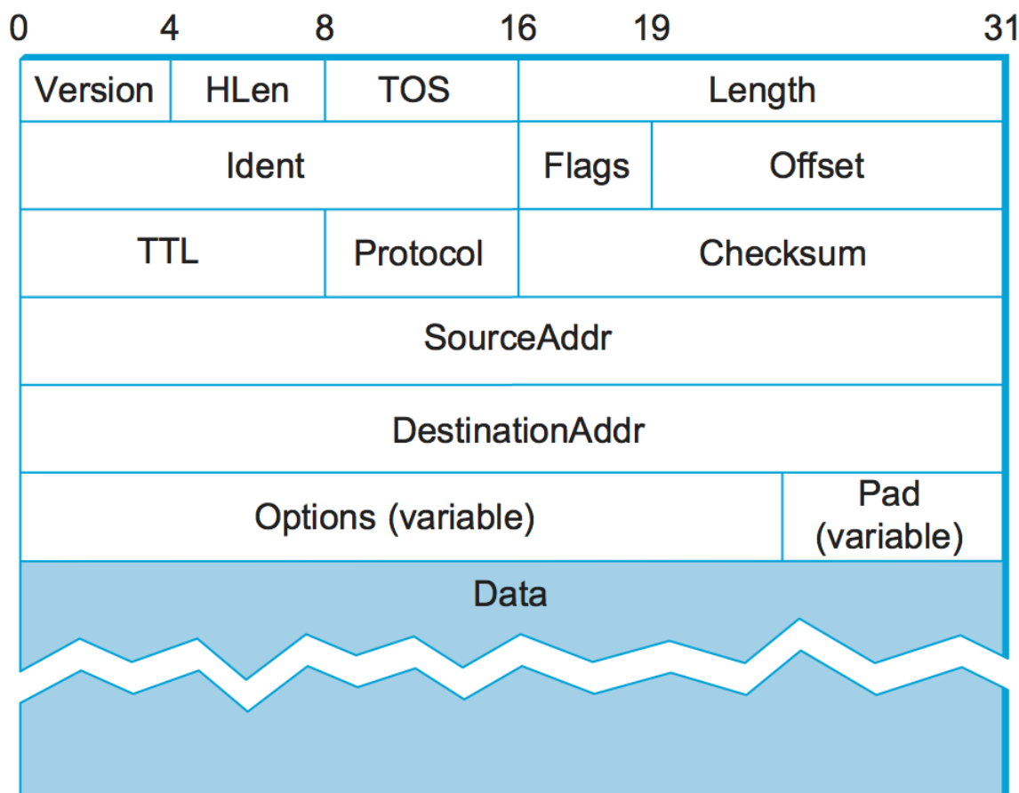
IPv4 packet header.
