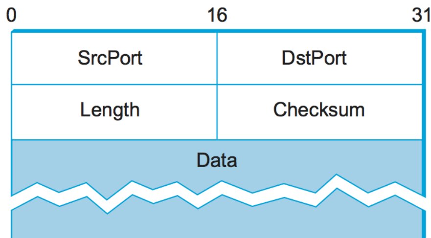
Format for UDP header.
