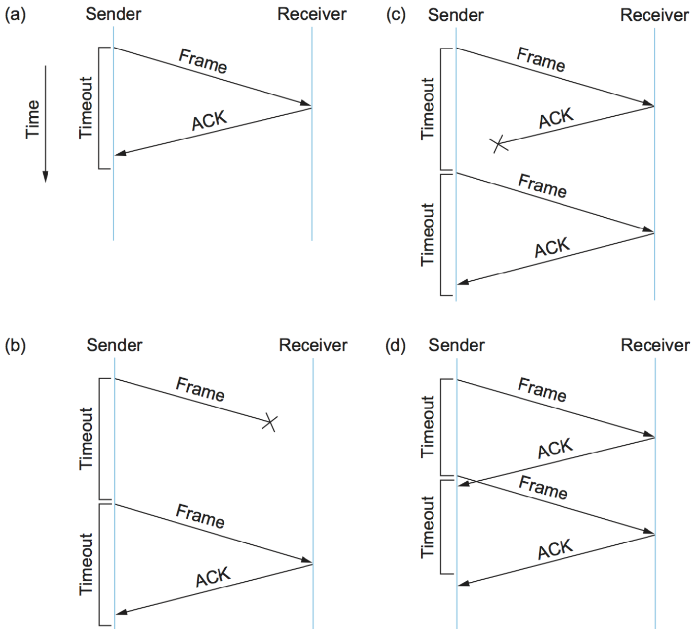
Timeline showing four different scenarios for the stop-and-wait algorithm. (a) The ACK is received before the timer expires; (b) the original frame is lost; (c) the ACK is lost; (d) the timeout fires too soon.
