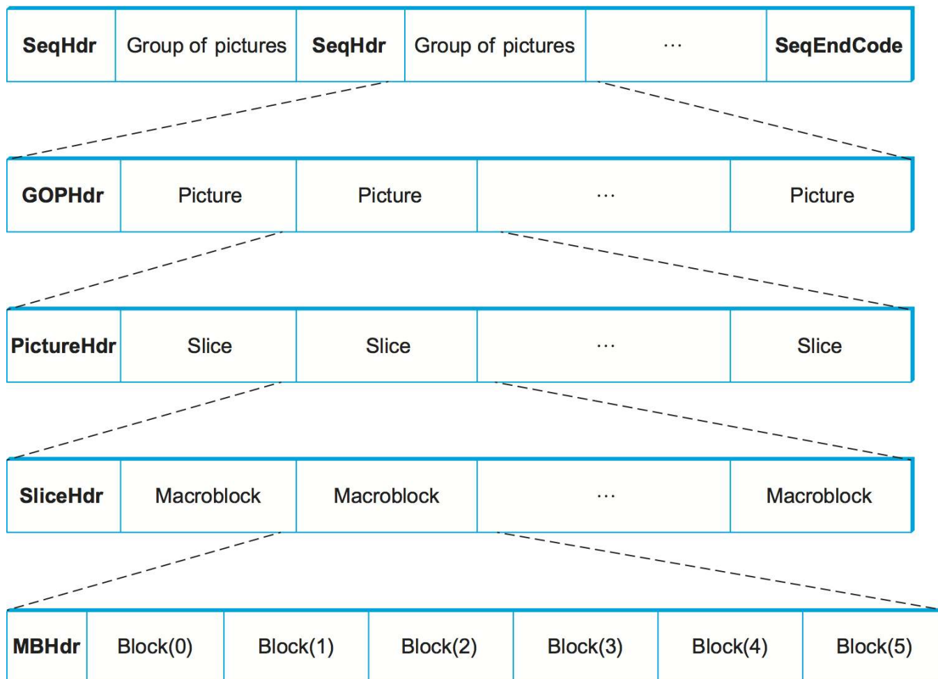
Format of an MPEG-compressed video stream.
