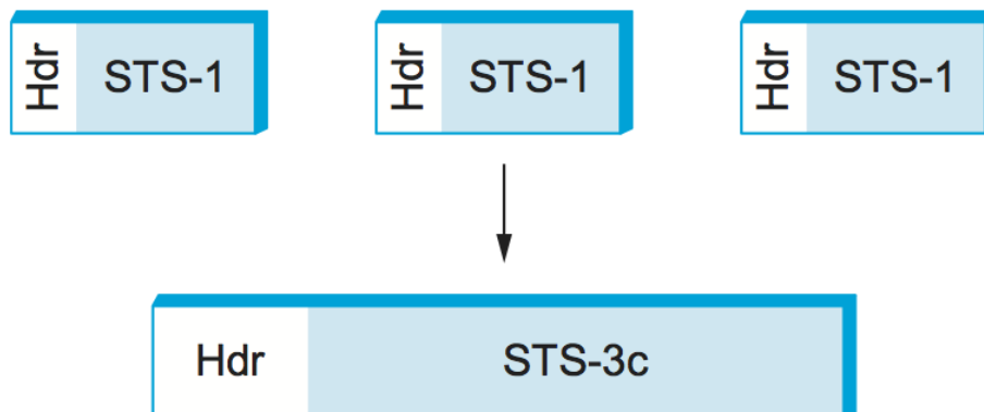
Three STS-1 frames multiplexed onto one STS-3c frame.
