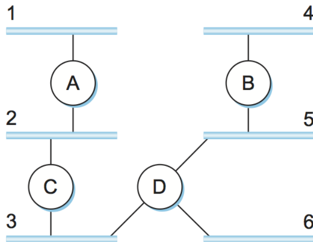
Example network running RIP.
