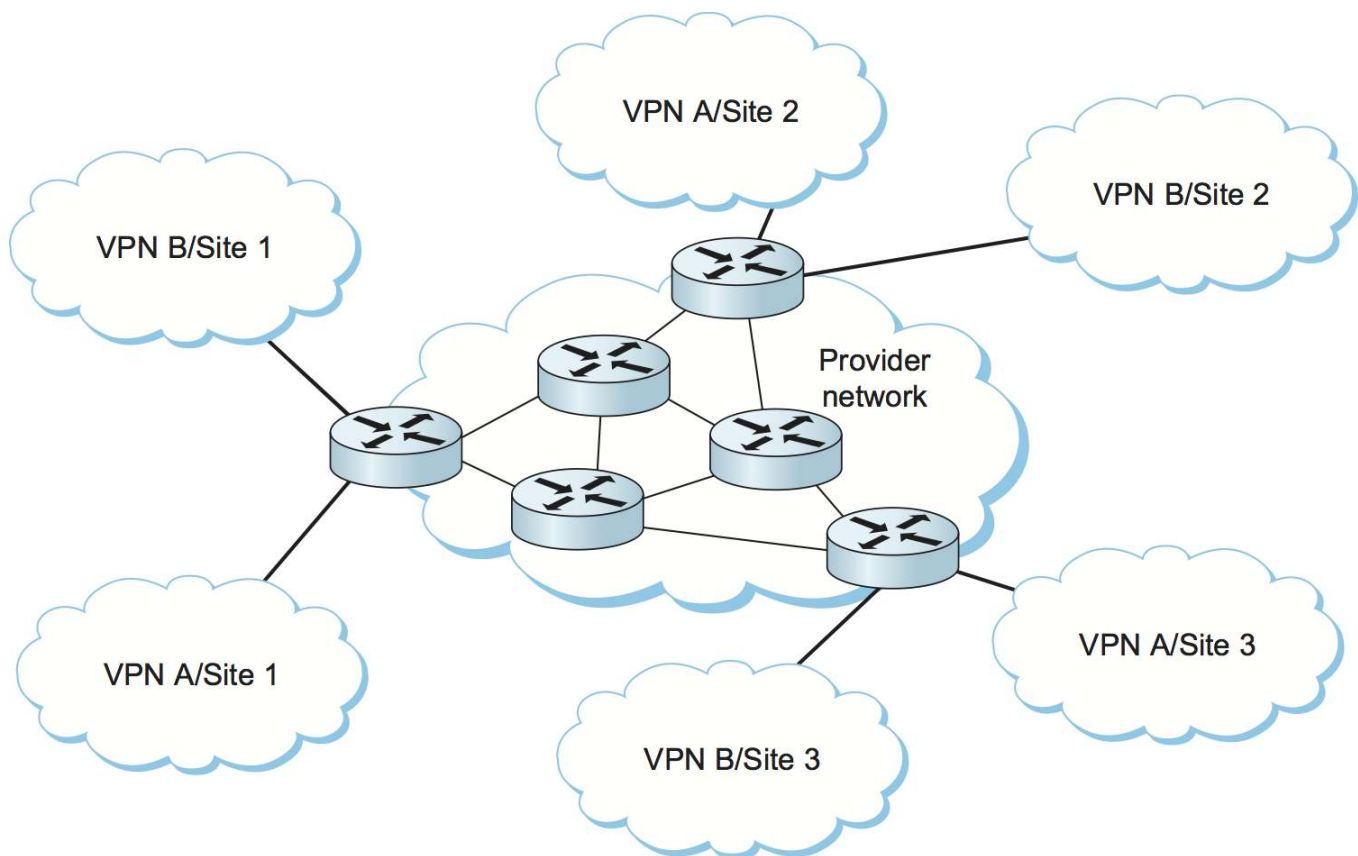
Example of a layer 3 VPN. Customers A and B each obtain a virtually private IP service from a single provider.
