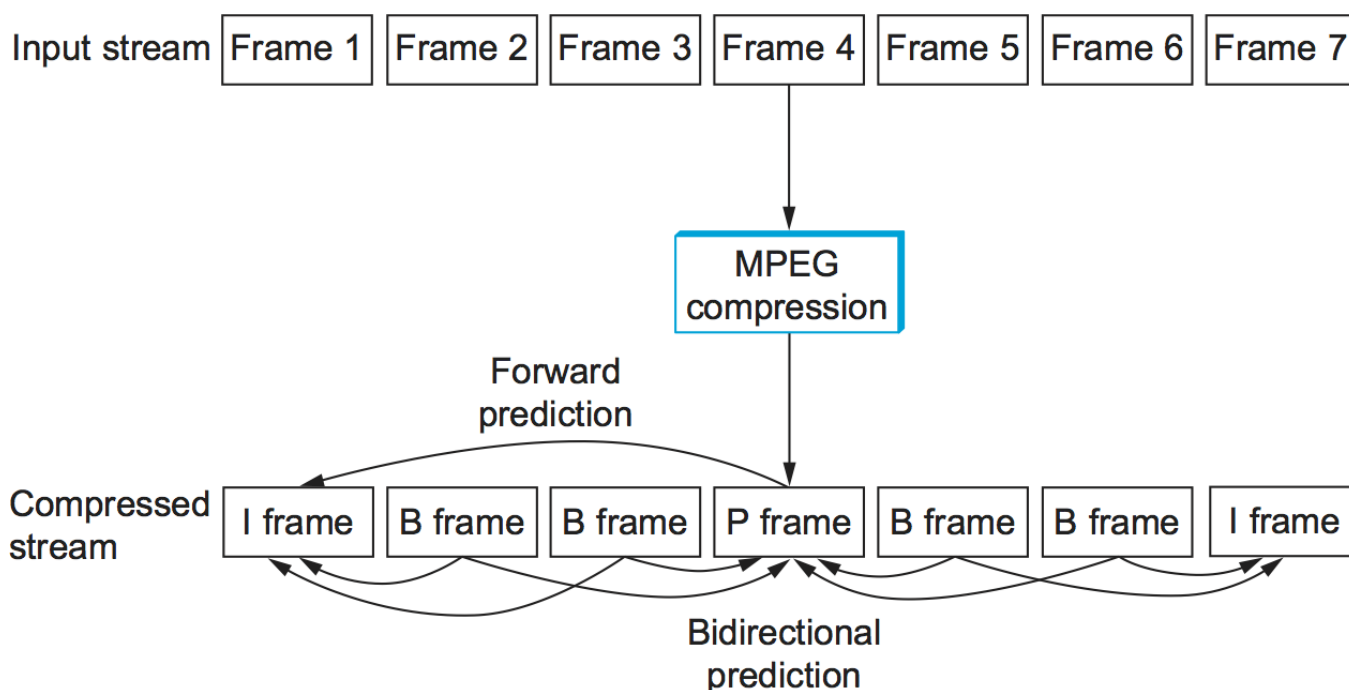
Sequence of I, P, and B frames generated by MPEG.
