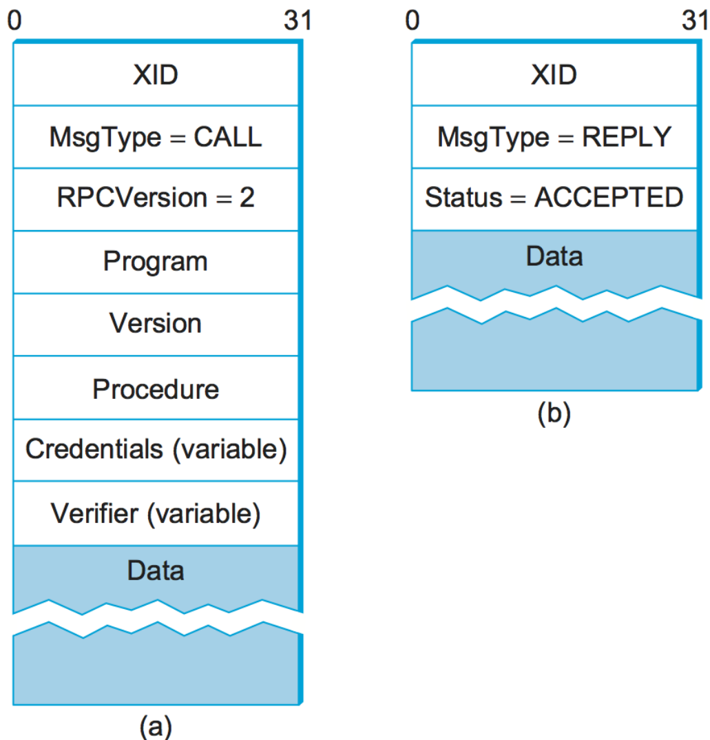
SunRPC header formats: (a) request; (b) reply.
