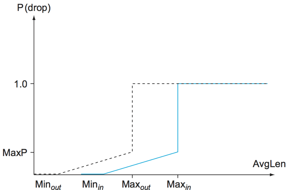
RED with In and Out drop probabilities.
