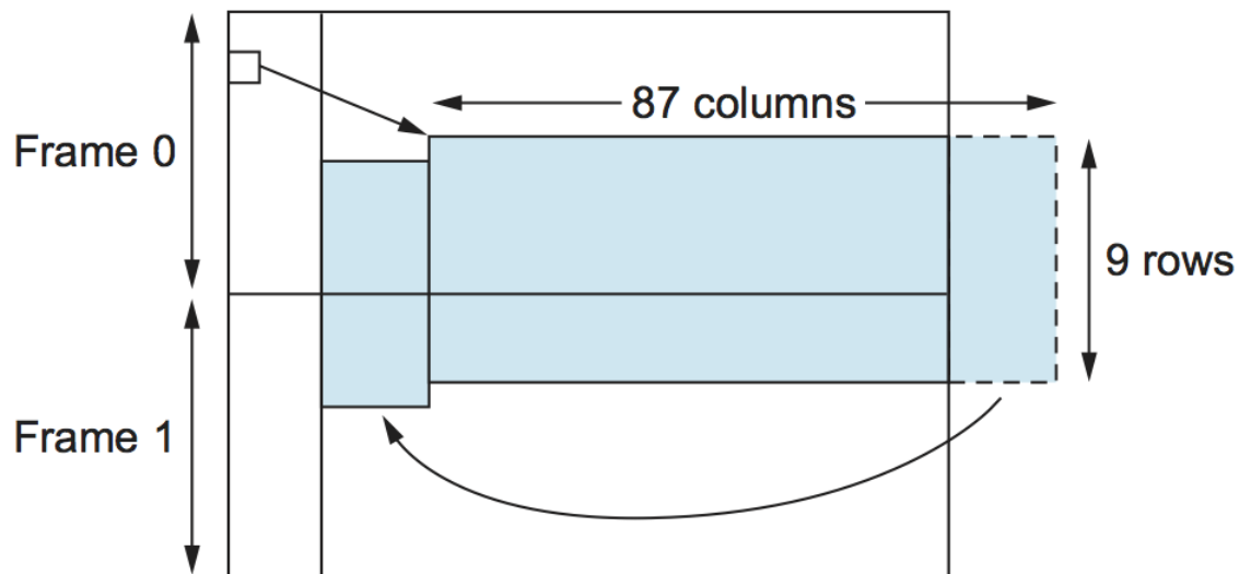
SONET frames out of phase.
