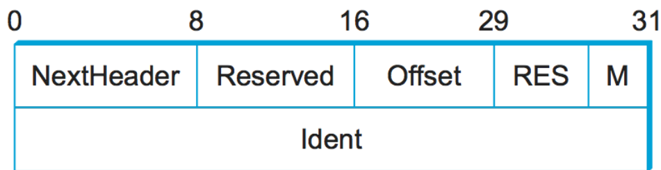
IPv6 fragmentation extension header.
