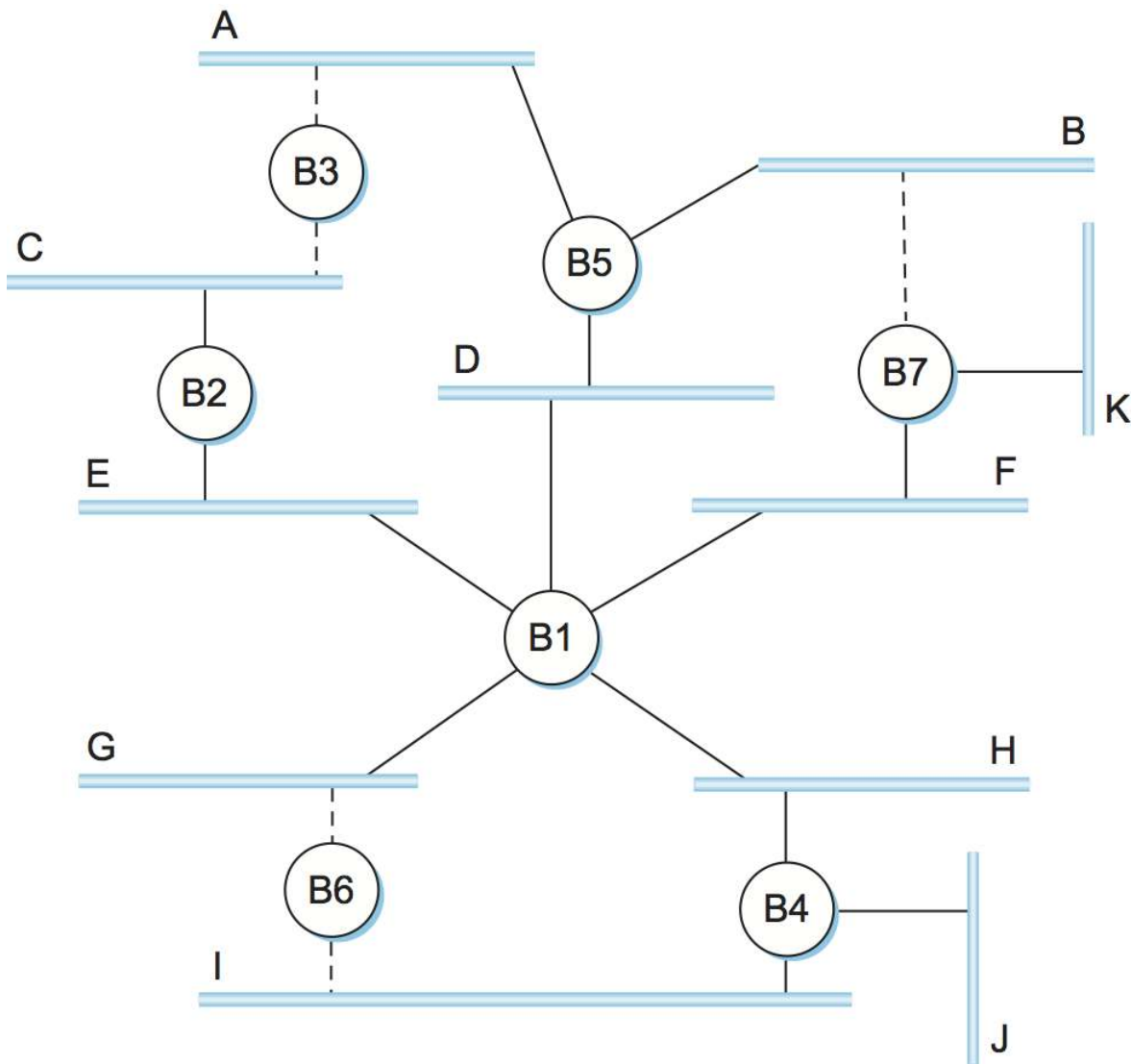
Spanning tree with some ports not selected.
