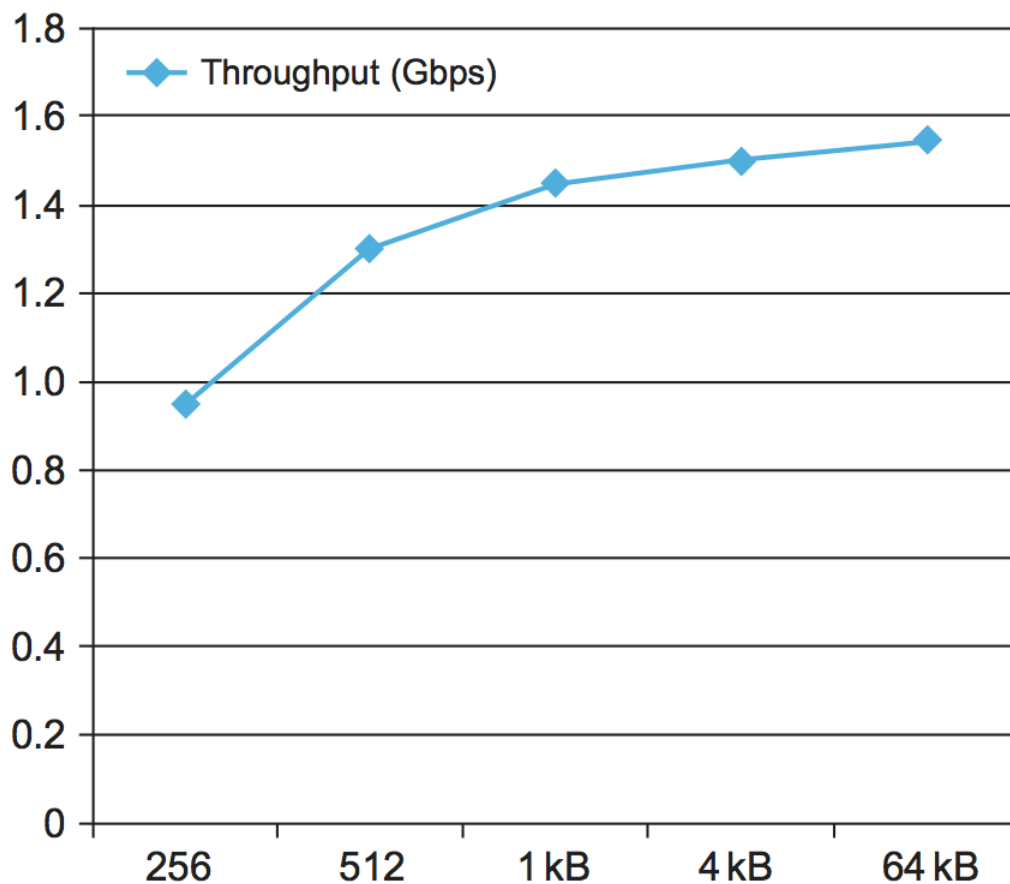
Measured throughput using TCP, for various message sizes.
