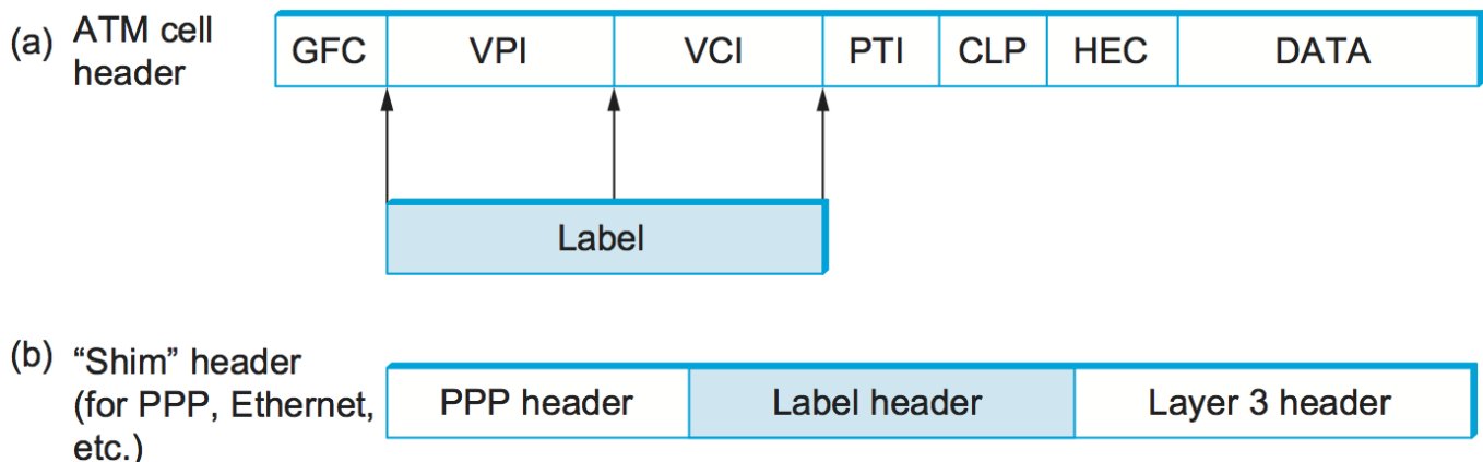
(a) Label on an ATM-encapsulated packet; (b) label on a frame-encapsulated packet.
