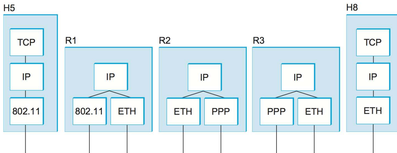
A simple internetwork, showing the protocol layers used to connect H5 to H8 in the above figure. ETH is the protocol that runs over the Ethernet.
