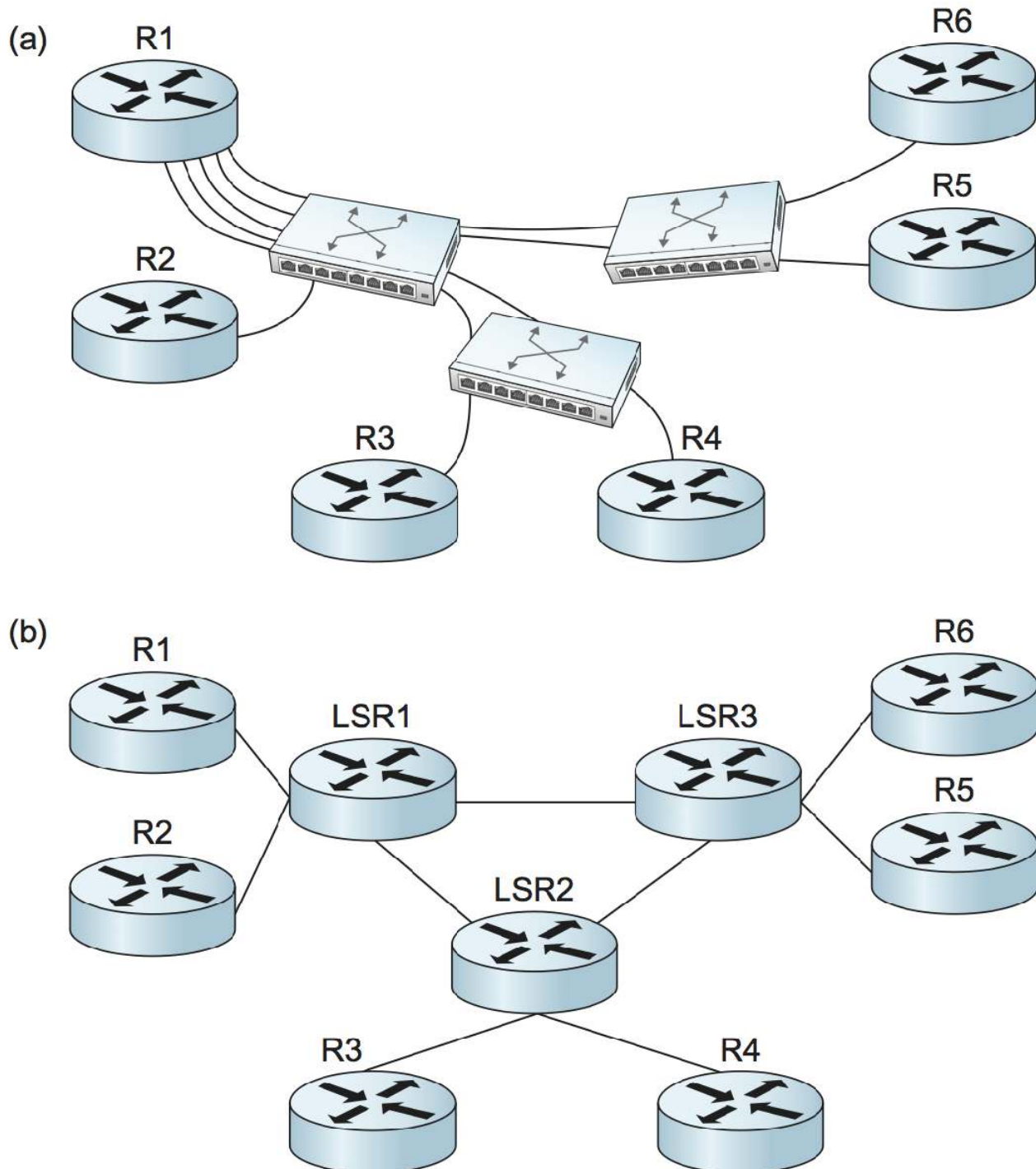
(a) Routers connect to each other using an overlay of virtual circuits. (b) Routers peer directly with LSRs.
