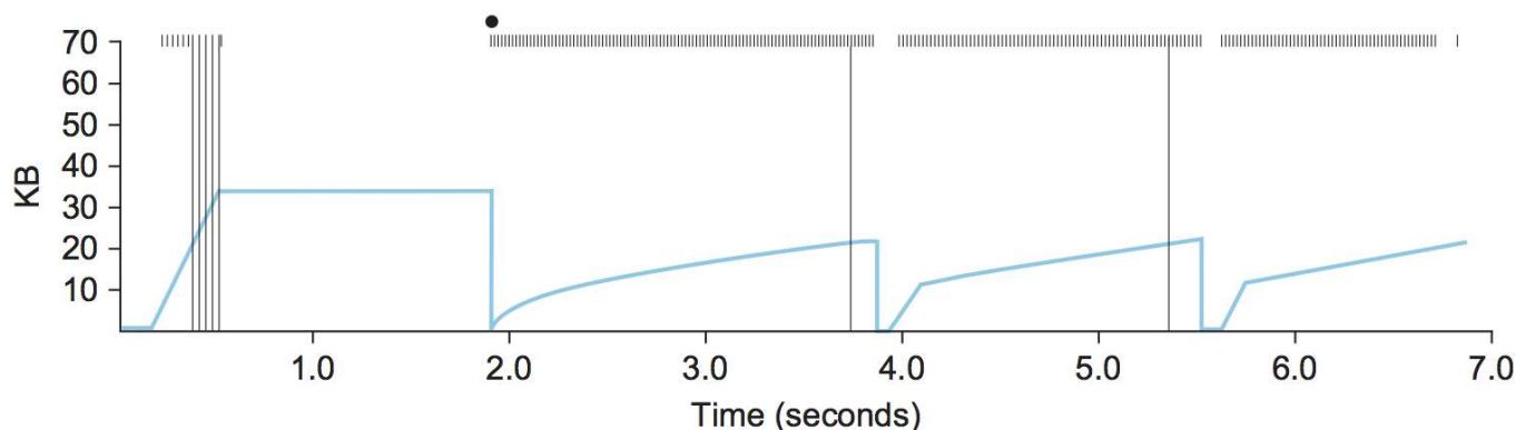
Trace of TCP with fast retransmit. Colored line = CongestionWindow; solid bullet = timeout; hash marks = time when each packet is transmitted; vertical bars = time when a packet that was eventually retransmitted was first transmitted.
