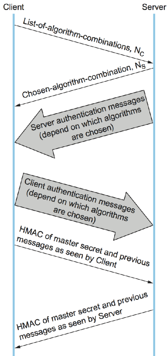
Handshake protocol to establish TLS session.
