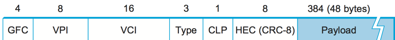
ATM cell format at the UNI.
