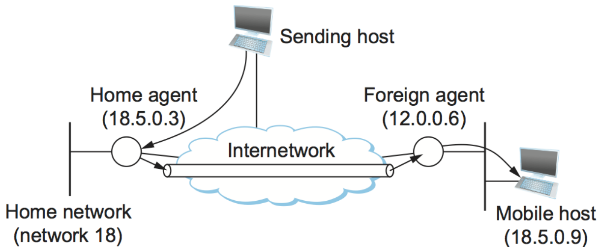
Mobile host and mobility agents.
