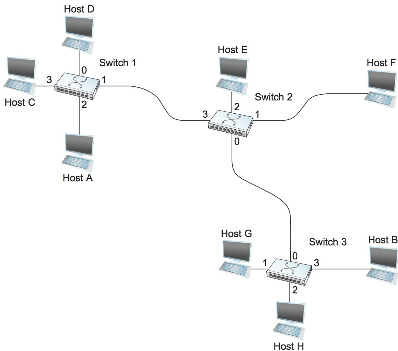
Datagram forwarding: an example network.
