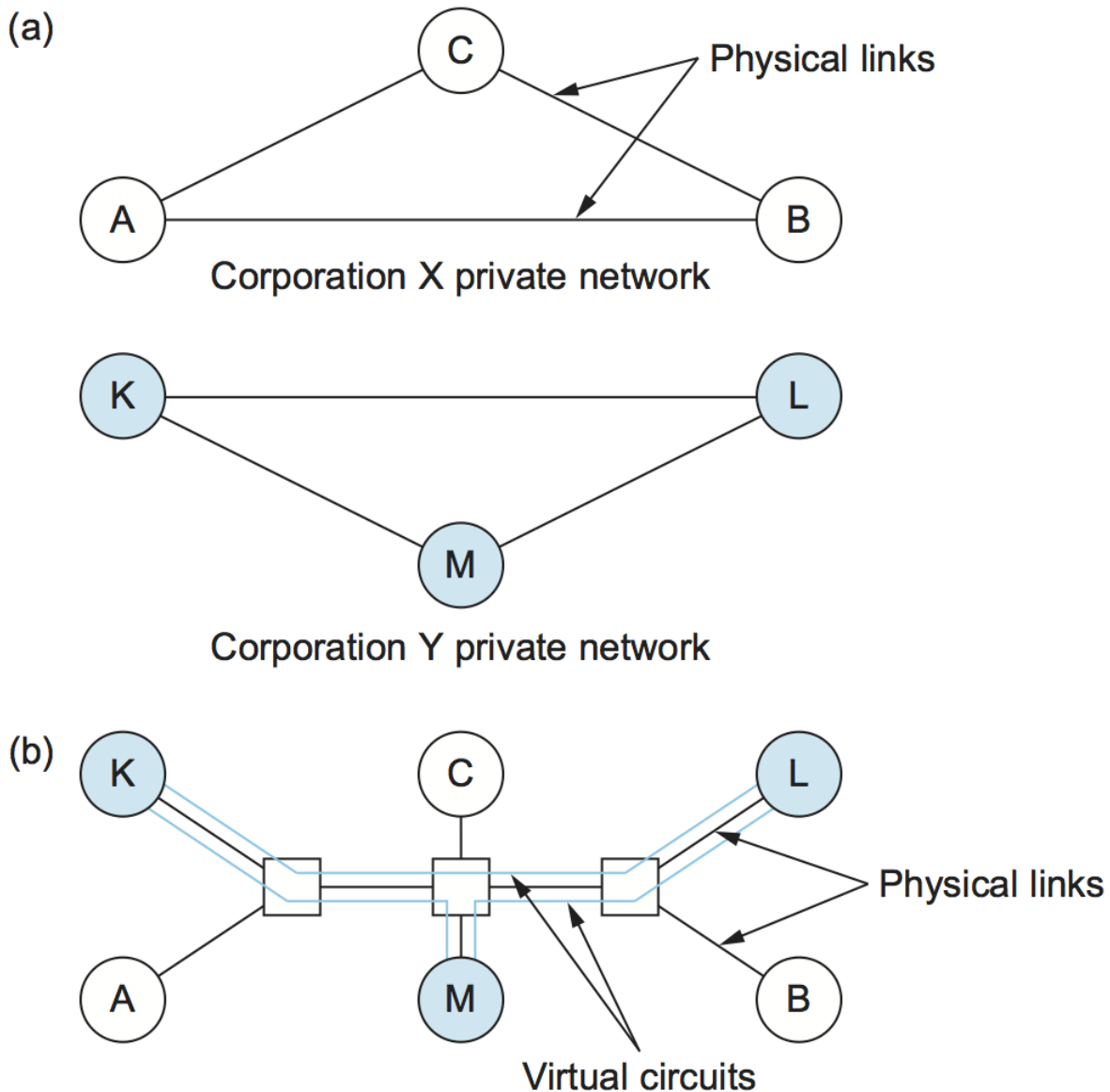
An example of virtual private networks: (a) two separate private networks; (b) two virtual private networks sharing common switches.
