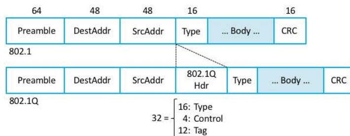
802.1Q VLAN tag embedded within an Ethernet (802.1) header.
