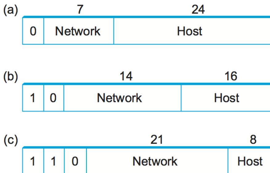
IP addresses: (a) class A; (b) class B; (c) class C.
