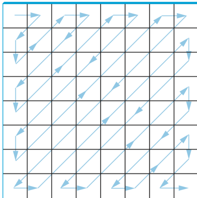
Zigzag traversal of quantized frequency coefficients.
