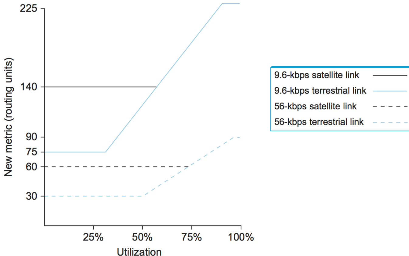
Revised ARPANET routing metric versus link utilization.
