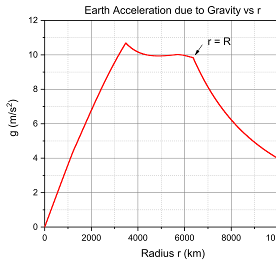
Figure 54.3: Modeled acceleration due to gravity for Earth.
