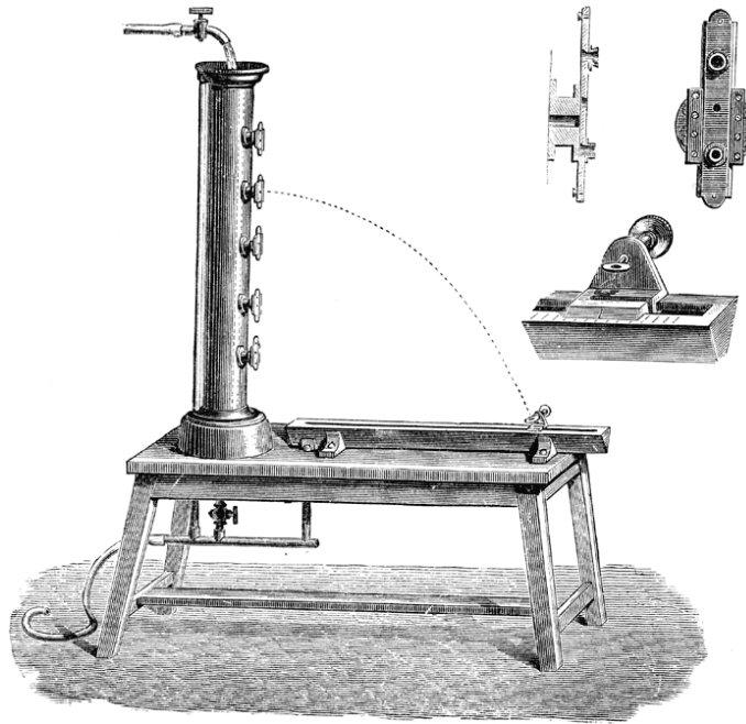
Figure 52.2: Apparatus for demonstrating Torricelli's theorem. (Ref. [16])
