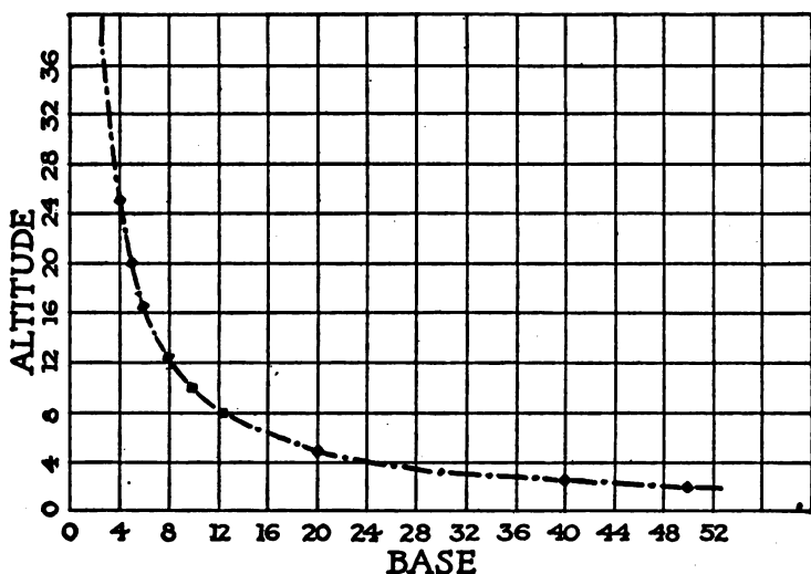
FIG. 139. The line shows the relationship between two numbers which vary INVERSELY ; in this case the relationship between the altitude and base of a rectangle whose area is constant, say 100 sq. ft. As the altitude INCREASES , the base DECREASES .
