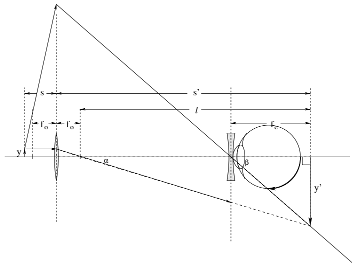
Figure 11.26: A “Galilean” microscope uses a diverging lens for the eyepiece. This does not affect the formula for the magnification, but it ensures that the eye sees the tiny objects erect instead of inverted. As always, we use a “central” ray for the second lens that is deflected at the plane of the first lens as if it passes through both lenses to find the location and size of the final image.
