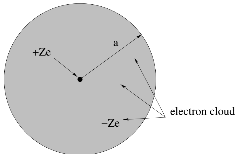
Figure 4.10: An “atom” consisting of a tiny massive nucleus surrounded by a uniform ball of negative charge modelling the “electron cloud”.
