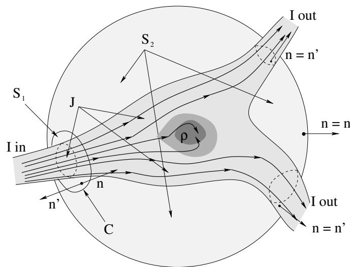
Figure 9.3: A very general current density flows through space. Some current flows in from the left and exits on the right, but some builds up in the current density \rho in the volume between the two surfaces S_1 and S_2 . The point is that the difference between the flux (current) in through S_1 and out through S_2 must be equal to the rate that charge builds up in between, because charge is conserved .
