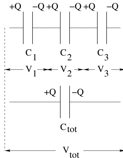
Figure 4.8: Find the total capacitance of a bunch of capacitors in series .
