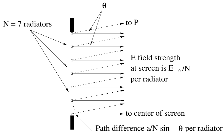
Figure 12.14: If we split the slit up into N radiators, the field amplitude at the maximum in the center of the screen from each radiator is E_0/N , where E_0 is the maximum amplitude from the entire slit there. When we consider the waves emerging at an angle \theta directed towards point P , each radiator travels an additional distance of \Delta r = \frac{a}{N} \sin(\theta) compared to the radiator immediately above it. Both of these relations scale with N , and hence will be useful when we try to let N \rightarrow \infty and fill in the entire slit with radiators.
