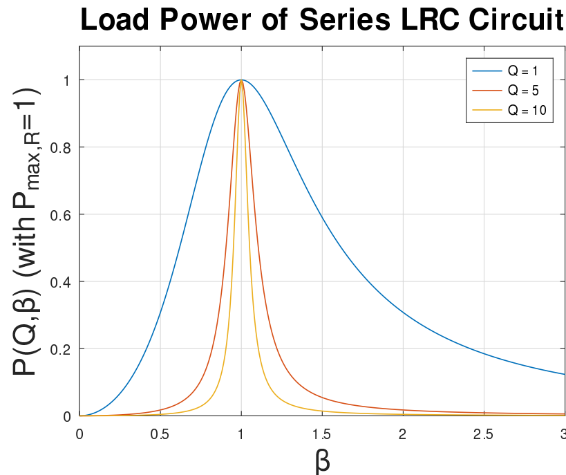
Figure 13.19: A typical series of resonance curves for Q = 1, 5, 10 , plotted on a scale such that \omega_0 = 1 , P_{\max} = 1 . This graph is universal and works for any values of P_{\max, R} , \omega_0 and an appropriately given or evaluated Q once one scales the abscissa and ordinate axes!
