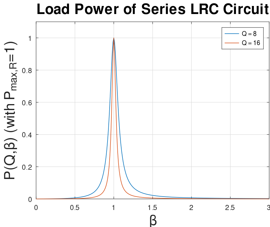
Figure 13.8: A graph of the dimensionless “filter function” for the two values Q = 8, 16 . This curve is exact (for P_{\max, R} = 1 )! One can obviously rescale the abscissa to make the location of ‘1’ any value \omega_0 desired and rescale the ordinate to correspond to any P_{R,\max} desired.
