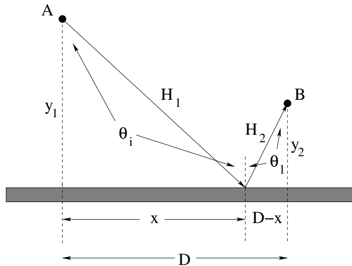
Figure 10.5: The path with \theta_i = \theta_l is the one with the minimal time when the entire trajectory is otherwise in a single medium with a constant speed.
