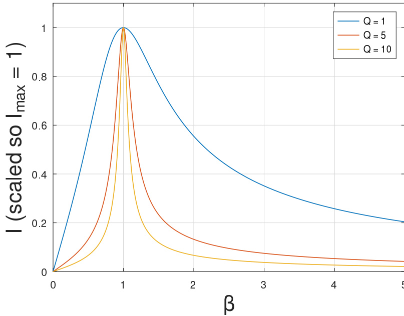
Figure 13.18: The amplitude I_0(\omega, \omega_0, Q) for several values of Q , on axes that can easily be scaled by I_{\max} and \omega_0 .
