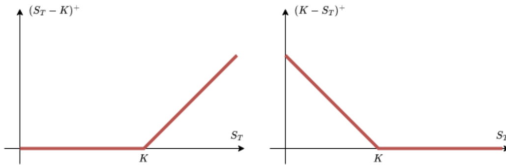
Figure 1: Payoff graphs for European call (left) and put (right) options with strike price K .
