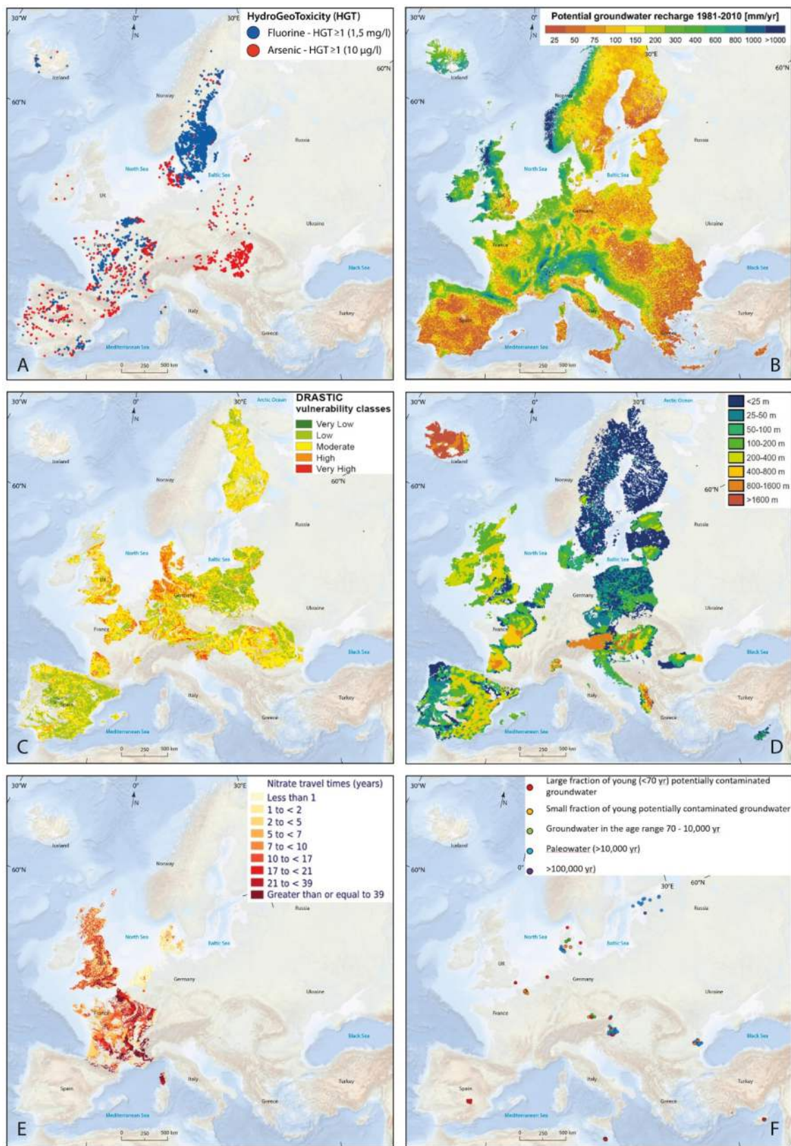
Fig. 4. Examples of groundwater quality and quantity data available in the EGD map viewer. (a) Groundwater As (red) and F (blue) concentrations above EU drinking water standards (Giménez-Forcada et al., 2022, EGD, 2023d), (b) Annual potential groundwater recharge as averaged for the period 1981–2010 (Martinsen et al., 2022, EGD, 2023e), (c) Groundwater vulnerability to pollution from the surface (DRASTIC Index, EGD, 2023f), (d) Thickness of exploitable aquifers (EGDI, 2023g, Andersen et al., 2023), (e) Nitrate travel time through the unsaturated zone (EGDI, 2023h) and (f) Groundwater age indicators in European aquifers – examples (EGDI, 2023i). (For interpretation of the references to colour in this figure legend, the reader is referred to the web version of this article.) Note! The user is able to choose from four different base maps as background layers in EGD. Here we have used the "EMODNet Bathymetry Basemap" as background.
