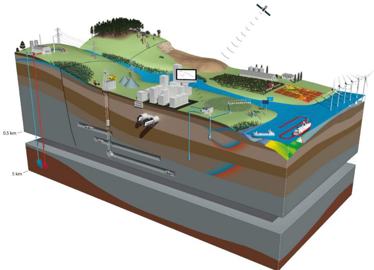
Fig. 1. Conceptual model of natural resources exploitation, remote and in-situ observations, mapping, and monitoring of Earth's natural resources, geohazards (illustrated by fault and landslide) and groundwater-dependent ecosystems. Red/Blue boundaries in the subsurface in the coastal zone are salt- (red) /freshwater (blue) boundaries, while red and blue wells to several kilometres' depth illustrate the use of deep geothermal energy. Coloured squares NW of windmills illustrate digital soil map. (For interpretation of the references to colour in this figure legend, the reader is referred to the web version of this article.)
