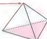
triangular-based pyramid
