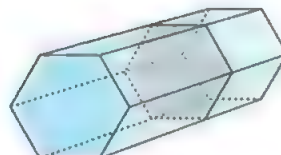
hexagonal prism
