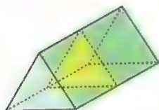
triangular prism
