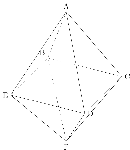
FIGURE 13.8 – Octaèdre ABCDEF
