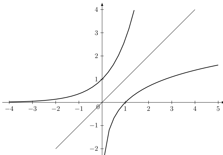
FIGURE 33.5 – Croissances comparées
