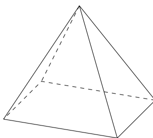
FIGURE 16.10 – Pyramide
