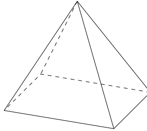
FIGURE 17.18 – Pyramide
