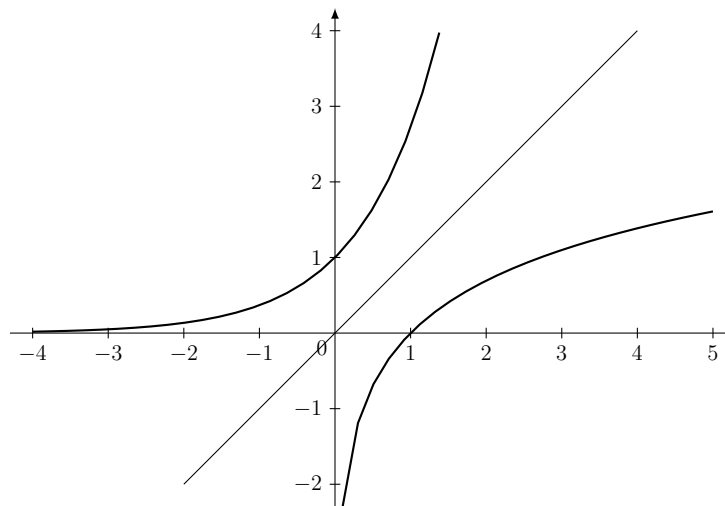
FIGURE 34.3 – Croissances comparées
