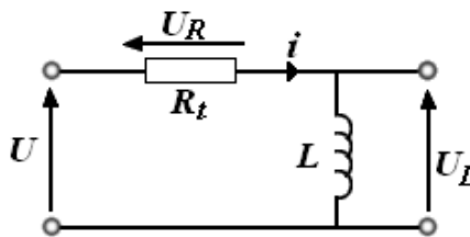
FIGURE 44.5 – Circuit RL
