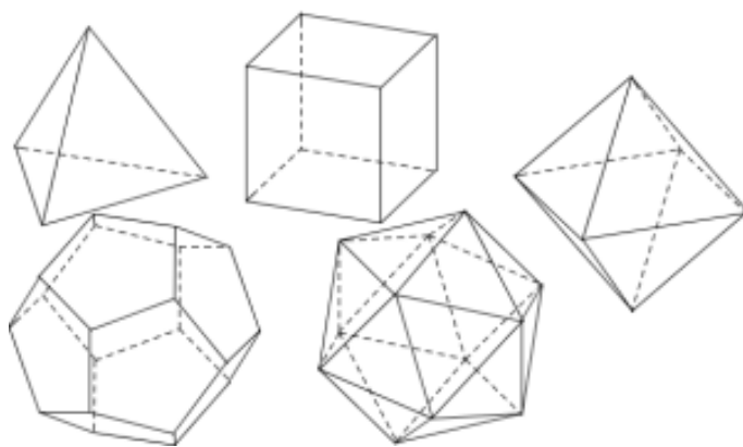
FIGURE 16.20 – Solides de Platon
