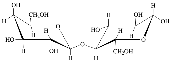
Lactose O - \beta -D-galactosyl-(1 \rightarrow 4)- \beta -D-glucose
