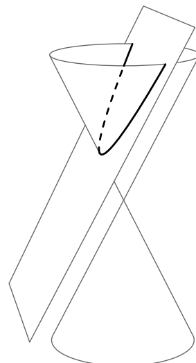
Parabole
