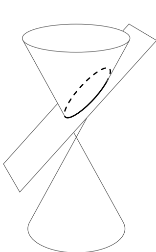
Ellipse
