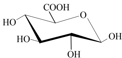
Acide \beta -D-glucuronique
