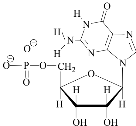
Guanylate [G]
