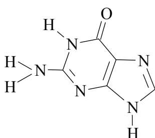
Guanine
