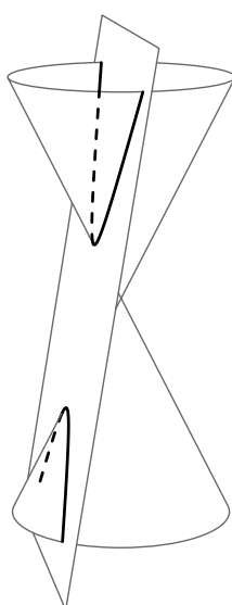
Hyperbole
