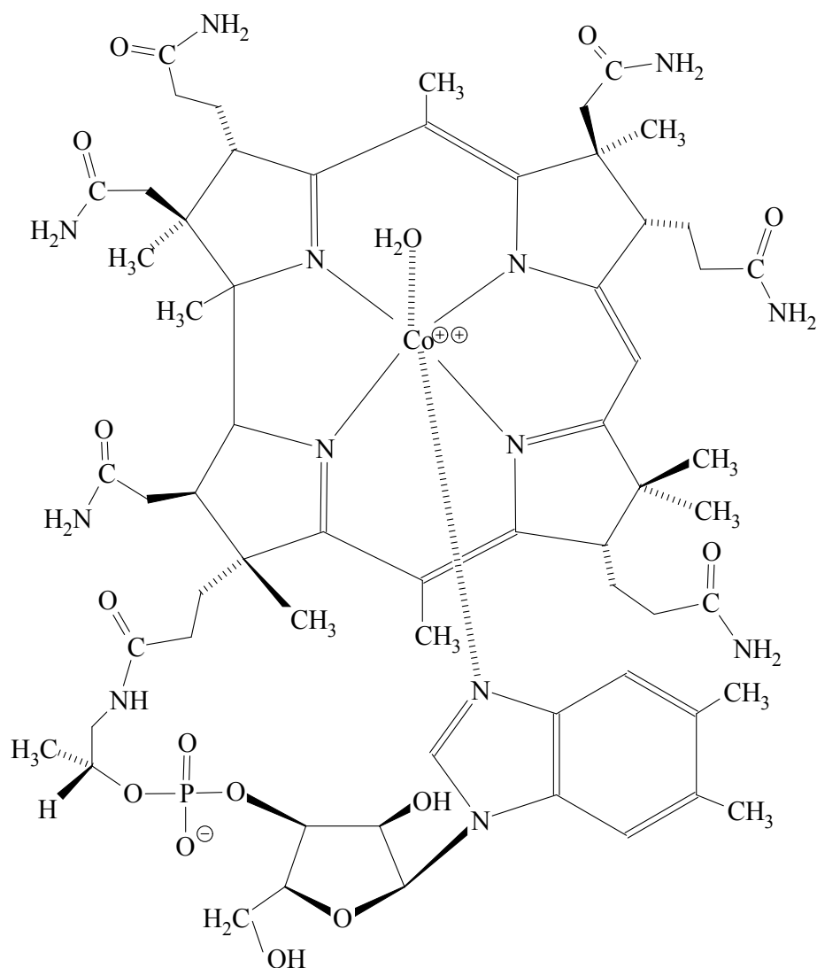
Cobalamine – vitamine B12
