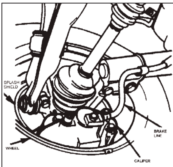
Figure 4 Illustrates a typical disc brake assembly for a front wheel drive vehicle.
