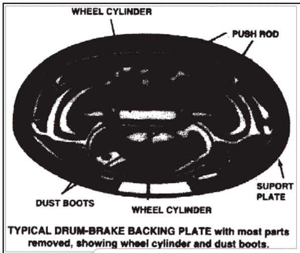
Figure 2 Shows a typical drum brake. When the drum is removed, the wheel cylinder should be checked for leakage, damaged, loose or missing parts, retention and dust boot condition.
